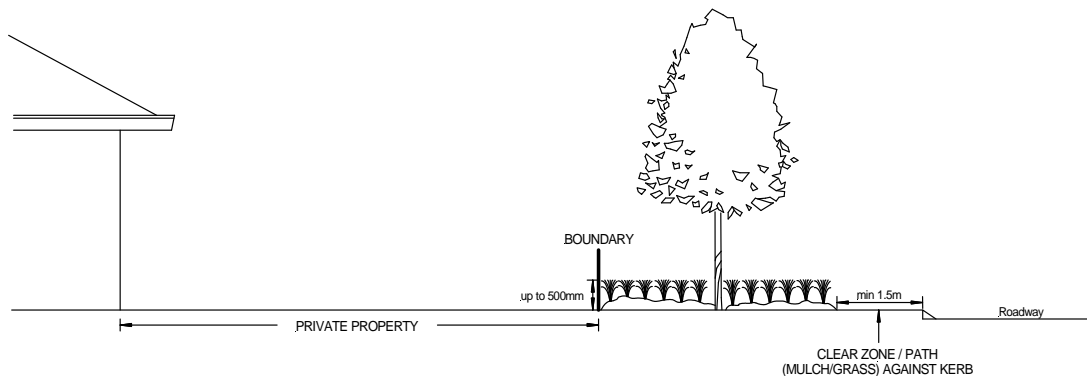
VERGE DEVELOPMENT - TYPICAL SECTION
