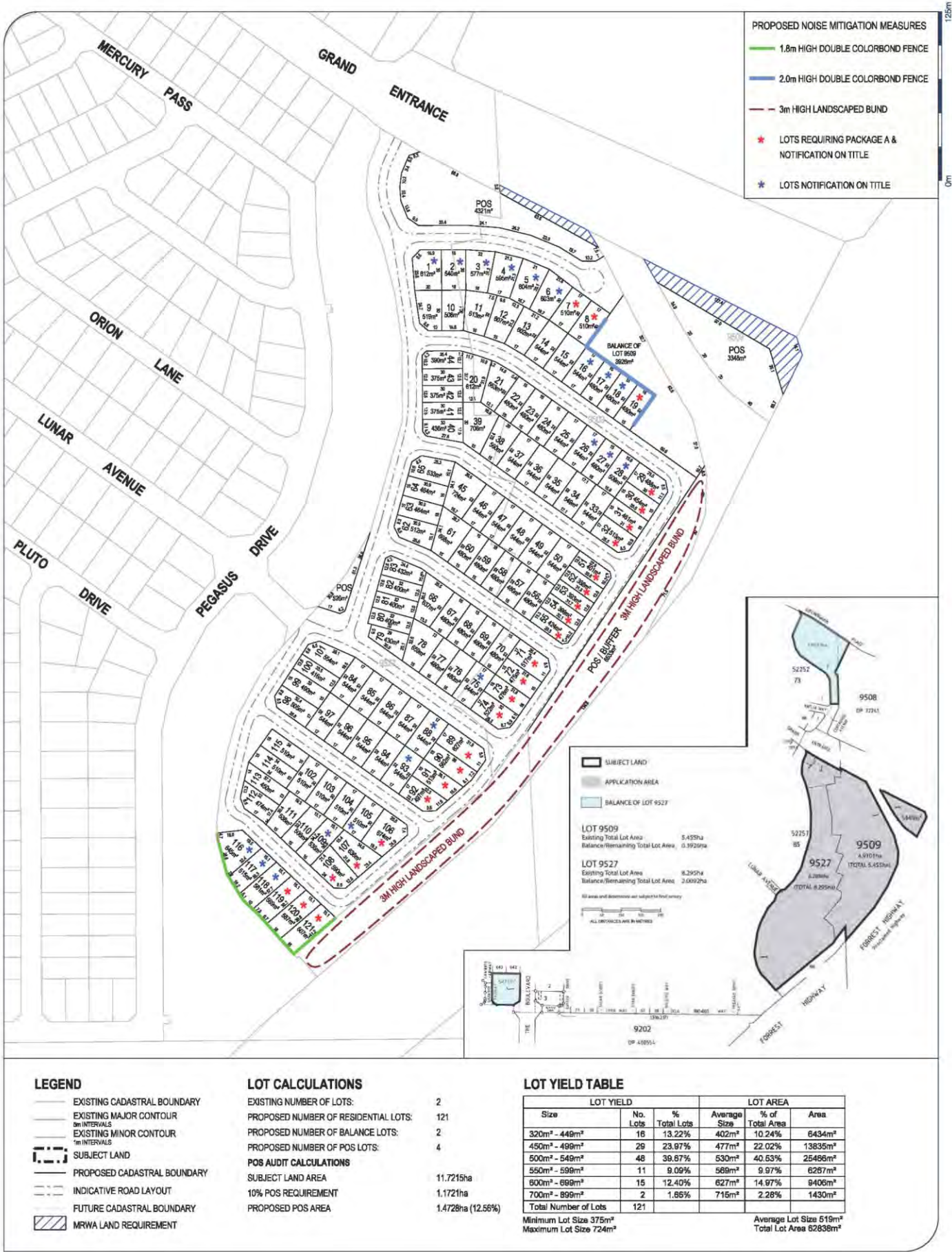
Figure 5 – Location of Noise Mitigation Measures
